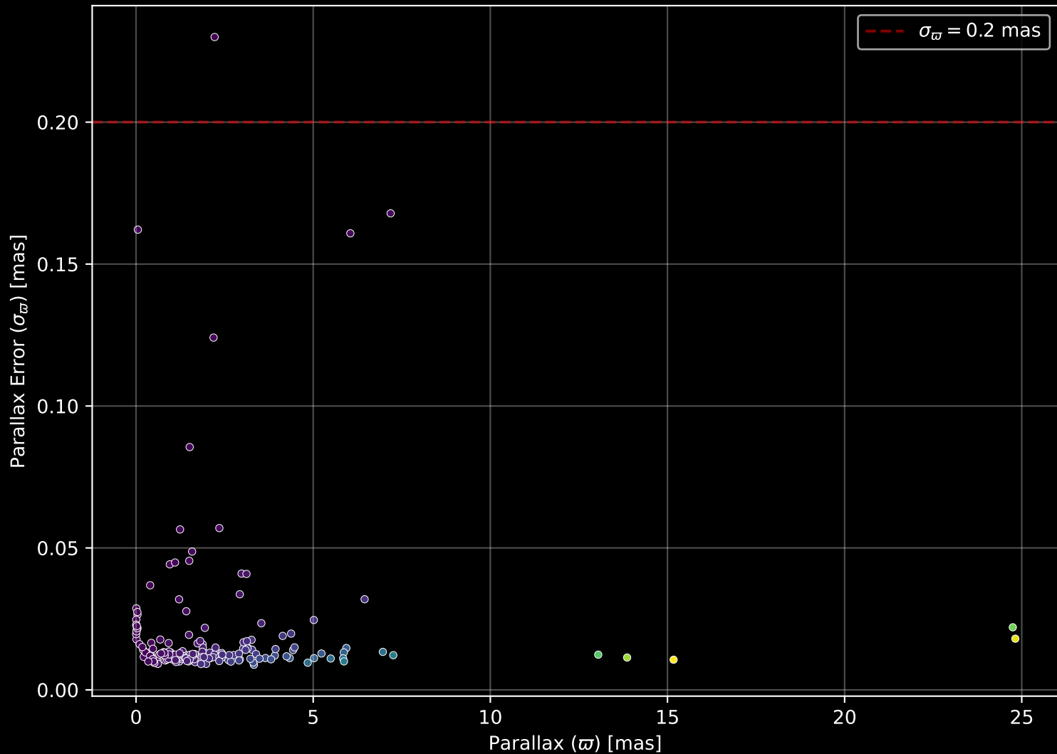
APOGEE DR17 Field: [280-27] Parallax Quality (n= 170)
