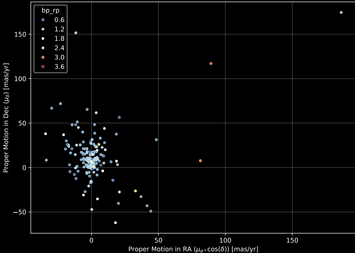
APOGEE DR17 Field: [280-27] Proper Motion Diagram (n= 170)
