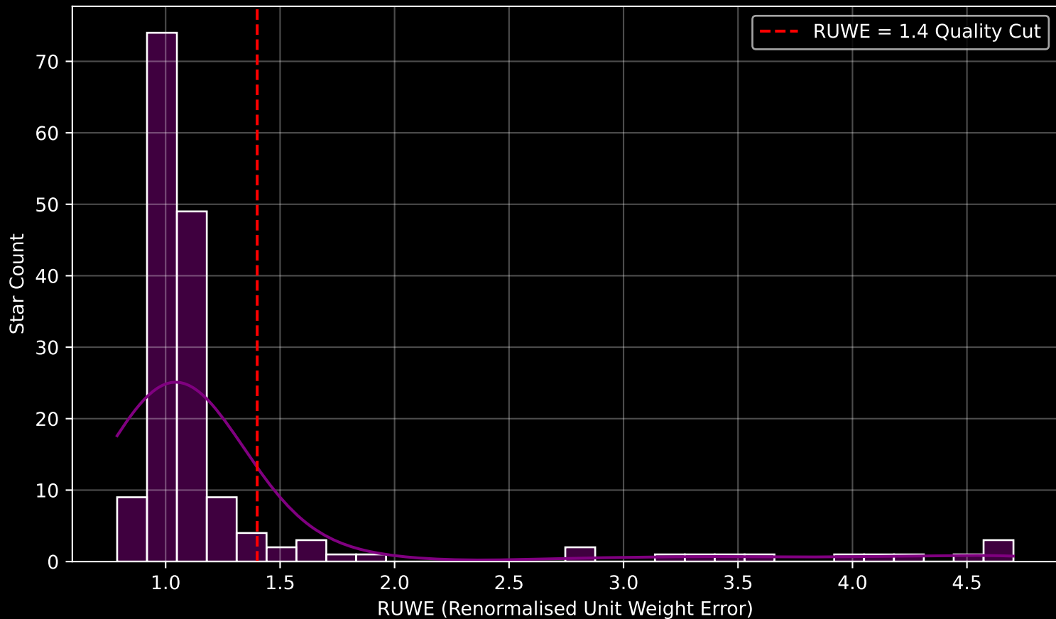
GAPOGEE DR17 Field [280-27] RUWE Distribution (n= 165)
