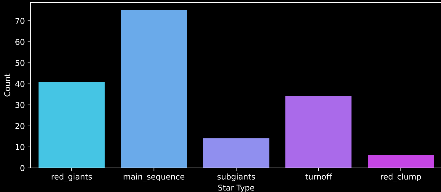
APOGEE DR17 Field: [280-27] Count plot of Star Type
